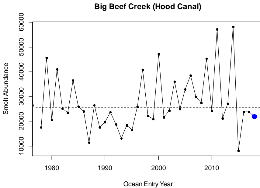
Figure 7. Time series of wild coho smolts from Big Beef Creek, ocean entry years 1978 to 2018. Blue point represents outmigration of the cohort included in this forecast. Horizontal line is the geometric mean of the time series.
