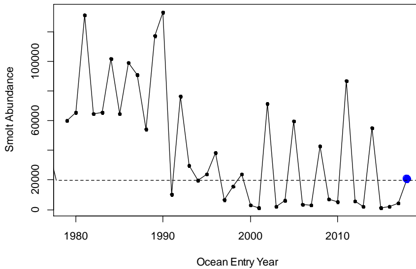
Figure 14. Time series of natural-origin coho smolts from the Deschutes River, ocean entry years 1979 to 2018. Blue point represents outmigration of cohort included in this forecast. Horizontal line is the geometric mean of the time series.
