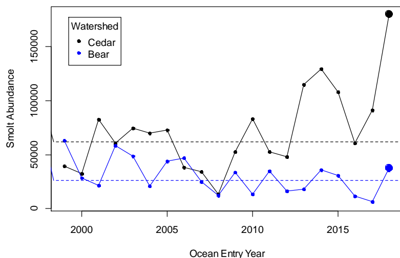
Figure 10. Time series of natural-origin coho smolts from Cedar River (black) and Bear Creek (blue), ocean entry years 1999 to 2018. Larger symbol represents outmigration of cohort contributing to this forecast. Horizontal lines are the geometric mean for the time series in each watershed.
