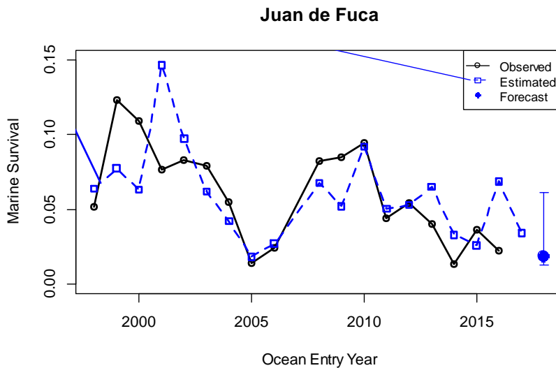
Figure 23. Marine survival of wild coho in the Strait of Juan de Fuca management unit, ocean entry year 1998 to 2017. Black solid line are the observed marine survivals. Blue dashed line are the marine survivals estimated by leave-one-out (jackknife) cross validation. Solid blue point is the forecasted marine survival ( \pm 90\% C.I) for the 2018 ocean entry year (2019 return year).
