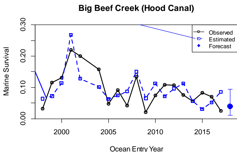
Figure 22. Marine survival of Big Beef Creek wild coho, ocean entry year 1998 to 2017. Black solid line are the observed marine survivals. Blue dashed line are the marine survivals estimated by leave-one-out (jackknife) cross validation. Solid blue point is the forecasted marine survival ( \pm 90\% C.I.) for the 2018 ocean entry year (2019 return year).
