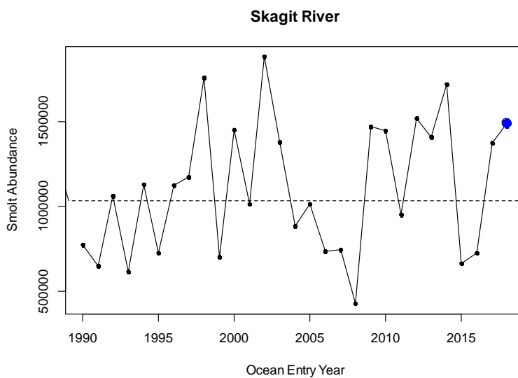
Figure 4. Time series of wild coho smolt outmigration from the Skagit River, ocean entry years 1990 to 2018. Blue point represents outmigration of the cohort included in this forecast. Horizontal line is the geometric mean of the time series.
