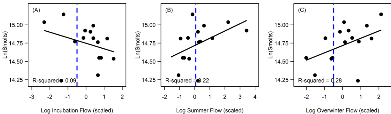
Figure 16. Chehalis River wild coho smolt production as a function of incubation flows (a), summer rearing flows (b), and overwinter rearing flows (c) for ocean entry year 2000-2018 as measured at USGS gage #12027500 in Grand Mound. Incubation flows are the cumulative daily mean flow between December 1 and March 1. Summer rearing flows are maximum daily flows in the month of August. Overwinter rearing flows are minimum daily flows between November 1 and February 28. Three data points were removed (OEY 2000, 2004, 2006) because of high leverage on the incubation flow regression. Vertical blue dashed line indicates the conditions associated with the 2018 ocean entry year.
