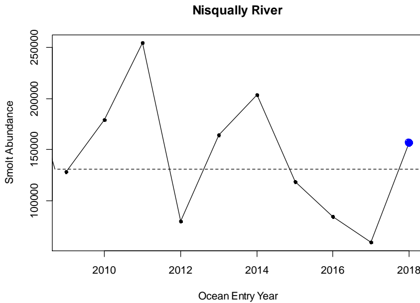
Figure 13. Time series of natural-origin coho smolts from the Nisqually River above the smolt trap (rm 12), ocean entry years 2009 to 2018. Blue point represents outmigration of the cohort included in this forecast. Horizontal line is the geometric mean for the time series.
