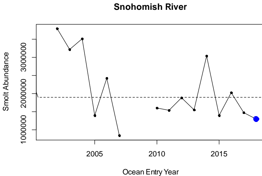
Figure 6. Time series of wild coho smolt outmigration from the Snohomish River, ocean entry years 2002 to 2018. No estimates are available for 2008 or 2009. Blue point represents outmigration of the cohort included in this forecast. The horizontal line is the geometric mean of the time series. Data provided by D. Holmgren (Tulalip Tribes).
