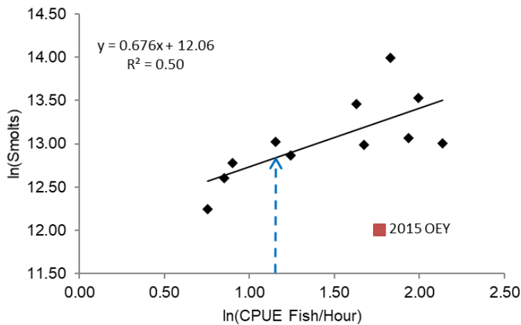
Figure 5. Correlation between CPUE of wild coho smolts in Stillaguamish smolt trap and back-calculated smolt estimates, 2003 to 2014. The 2015 ocean entry year was not used in the regression model. Dashed blue line corresponds to the 2018 ocean entry year. Smolt trap data were provided by K. Konoski (Stillaguamish Natural Resources).
