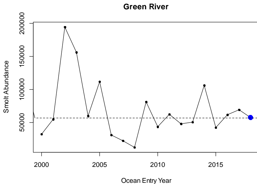
Figure 11. Time series of natural-origin coho smolts above the Green River smolt trap (river mile 34), ocean entry years 2000 to 2018. Blue point represents cohort contributing to this forecast. Horizontal line is the geometric mean for the time series.
