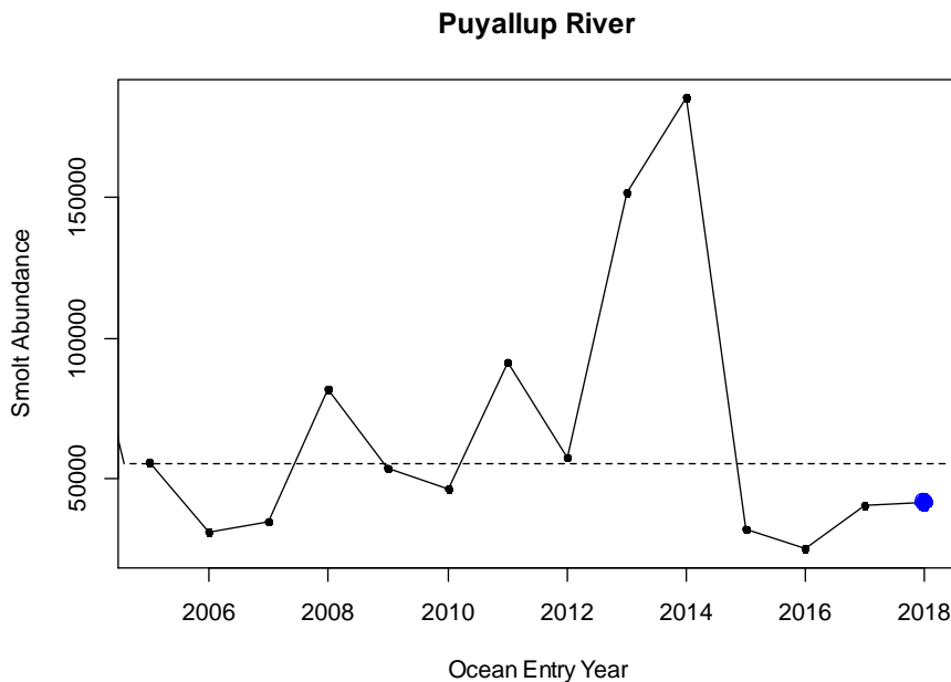
Figure 12. Time series of natural-origin coho smolts above the Puyallup River smolt trap (upstream of confluence with White River), ocean entry years 2005 to 2018. Blue point represents cohort included in this forecast. Horizontal line is the geometric mean of the time series. Data provided by Andrew Berger (Puyallup Tribe).
