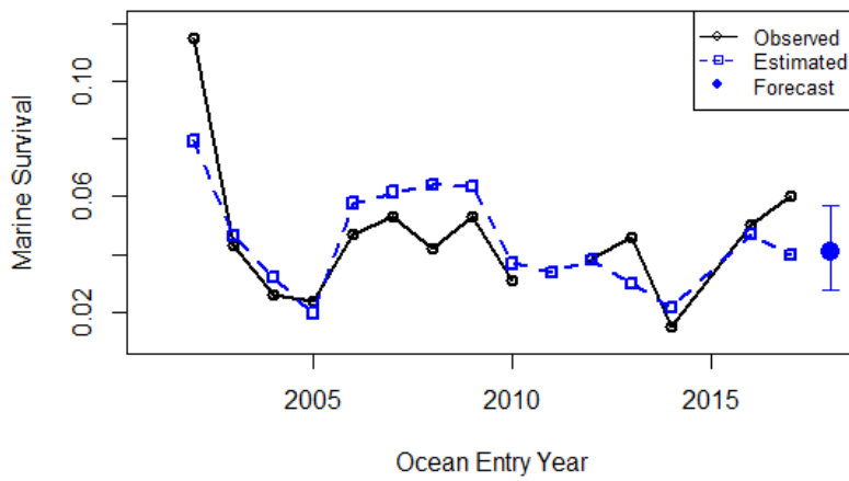
Figure 25. Marine survival of natural origin coho from the Lower Columbia River management unit, ocean entry year 2002 to 2018 (no data available for 2011). Black solid line are the observed marine survivals. Blue dashed line are the marine survivals estimated by leave-one-out (jackknife) cross validation. Solid blue point is the forecasted marine survival ( \pm 90\% C.I.) for the 2018 ocean entry year (2019 return year).
