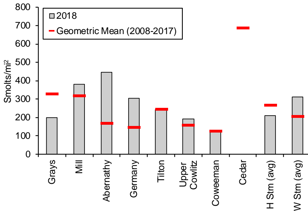
Figure 17. Coho smolt densities (smolts per mile 2 of watershed area) in eight Lower Columbia tributaries in Washington State. Graphs shows the 2018 density (bars) relative to the average smolt abundance from these watersheds (2008-2017).
