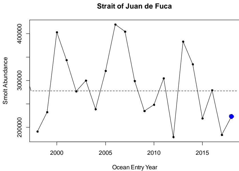
Figure 8. Time series of wild coho smolts from Strait of Juan de Fuca tributaries, ocean entry years 1998 to 2018. Blue point represents the cohort contributing to this forecast. The horizontal line is the geometric mean of the time series. Data provided by Hap Leon (Makah Tribe).
